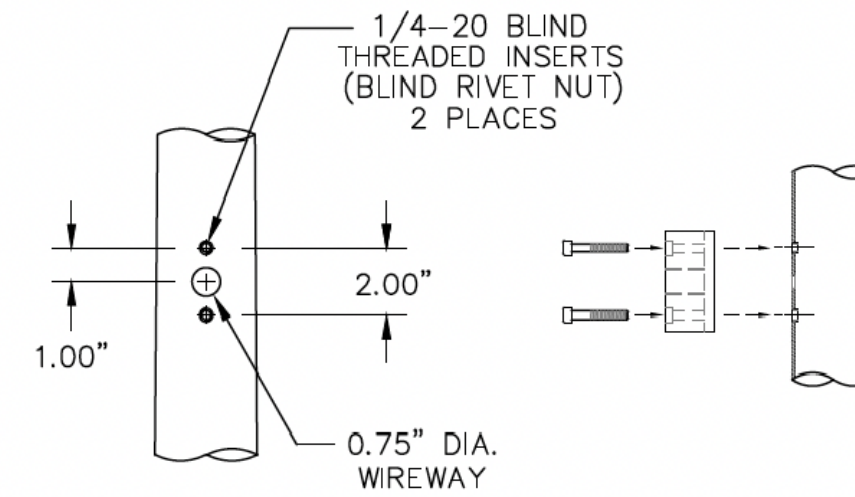
79511 INSERT/WIREWAY DETAIL
